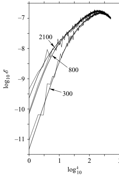
FIGURE 6. Actual energy spectra at t = 300, 800 and 2100 (thin lines) compared to hybrid-equipartition spectra (bold lines).
