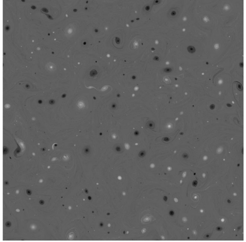
FIGURE 11. Vorticity \omega(\mathbf{x}, t) at t = 6 (a) and t = 24 (b) in one representative simulation. A linear greyscale is used from the minimum (black) to maximum (white) values.
