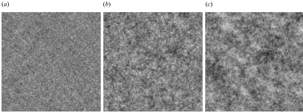
FIGURE 5. Streamfunction \psi(\mathbf{x}, t) at t = 200, 500 and 2000 (a–c). A linear greyscale is used from the minimum (black) to maximum (white) values.
